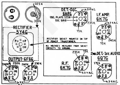
Fig. 1—Socket Voltages Measured from Underside of Chassis
