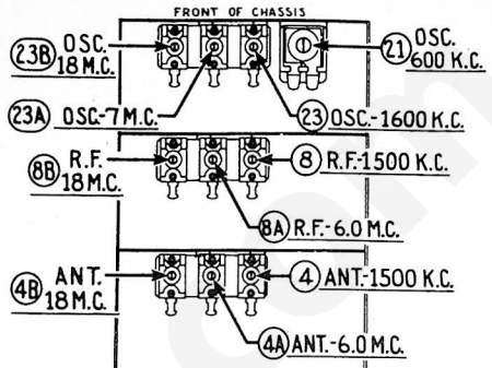
Fig. 7—Locations of R. F. Compensators
