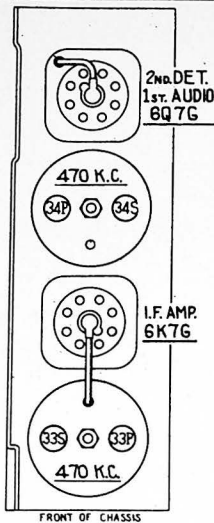
Fig. 6—Location of I. F. Compensators
