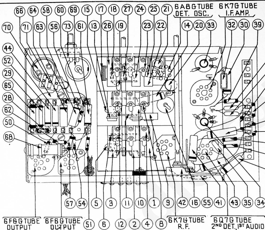
Fig. 4—Base View
